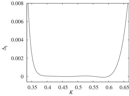
FIG. 1. Difference \Delta_l \equiv (C_{LTE} - C_{fit})/k between the specific heat of the Ising model as obtained from the low-temperature series of the energy and from the present least-squares analysis according to Eq. (16). The difference \Delta_l is at most 10^{-4} in the interval 0.39 < K < 0.60 .
