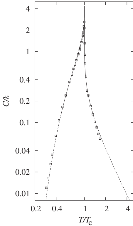
FIG. 3. Specific heat of the Ising model on the simple-cubic lattice. Logarithmic scales are used because of the large variation in the specific heat with temperature. The data points are existing experimental results [9] for \text{Rb}_3\text{CoCl}_5 . The full line represents the scaling form Eq. (16) with the parameters defined in Table I. The dashed lines at the lower left and right are obtained from low- and high-temperature series expansions [15,16] of the free energy.
